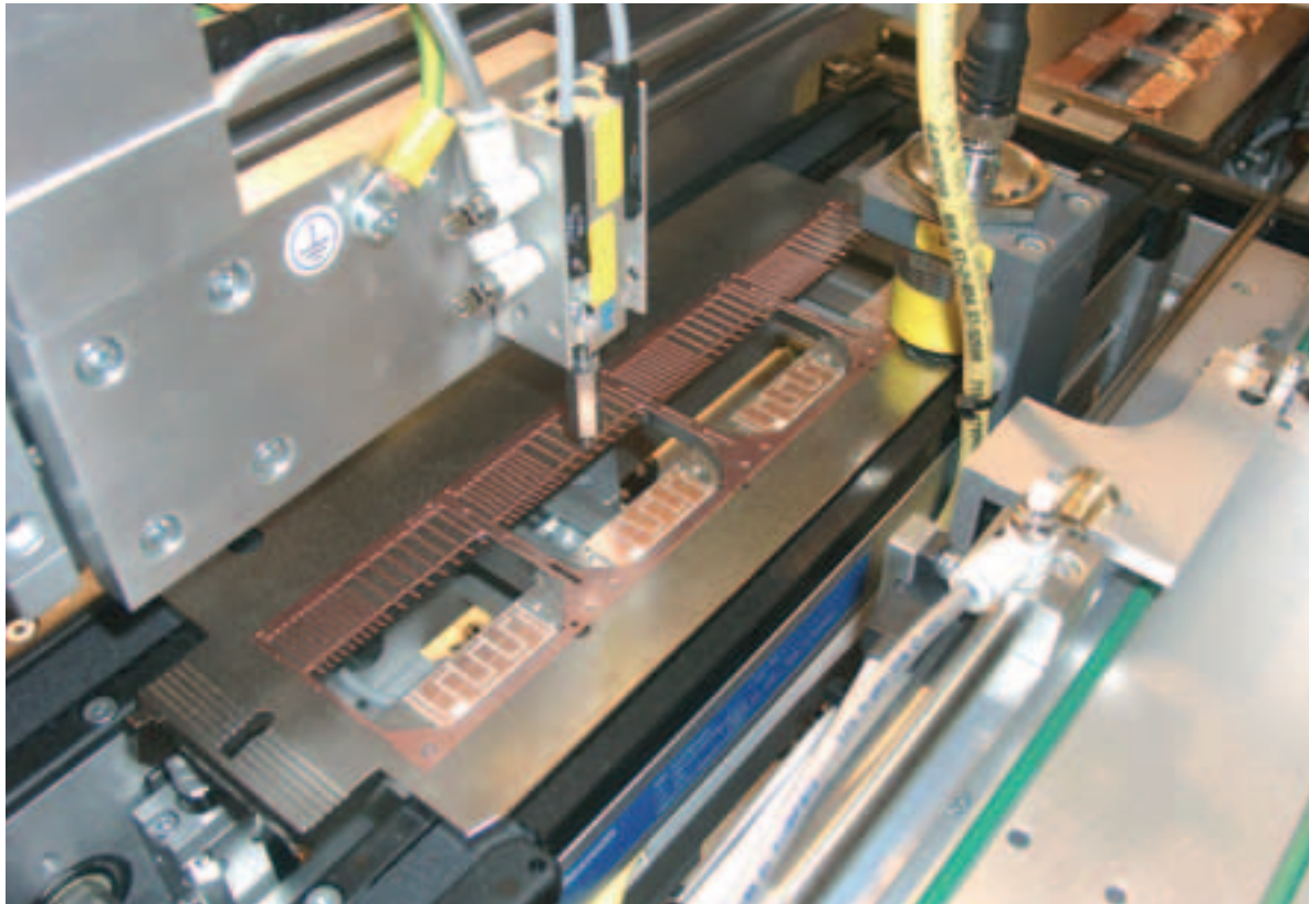
The complete placement and processing of parts is documented on the data carrier (in the photo under the yellow read-write head) in the parts carrier
